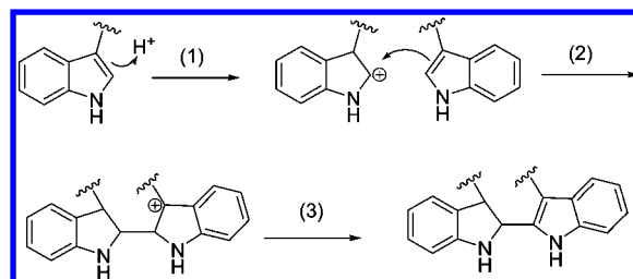
Figure 32. Mechanism of Trp dimerization: (1) protonation, (2) nucleophilic attack, and (3) elimination.
