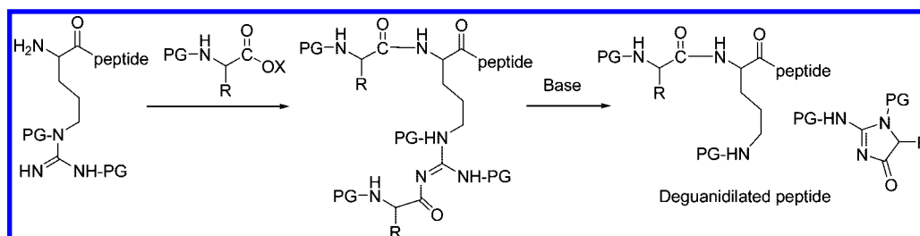
Figure 17. Acylation of the side chain of Arg during amino acid coupling, followed by base-catalyzed deguanidination. Adapted with permission from ref 290. Copyright 1984 Elsevier.
