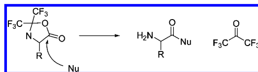
Figure 4. Deprotection of a HFA-protected amino acid via nucleophilic attack.
