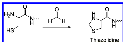
Figure 21. Thiazolidine formation by reaction of N -terminal Cys with formaldehyde.
