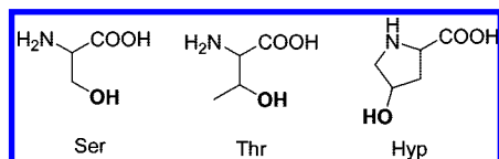
Figure 27. Serine (Ser), Threonine (Thr), and Hydroxyproline (Hyp).
