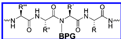
Figure 10. Partially backbone-protected peptide; BPG = backbone-protecting group.
