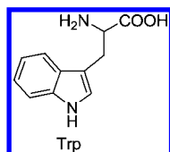
Figure 30. Tryptophan (Trp).
