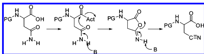
Figure 14. Dehydration of Asn.
