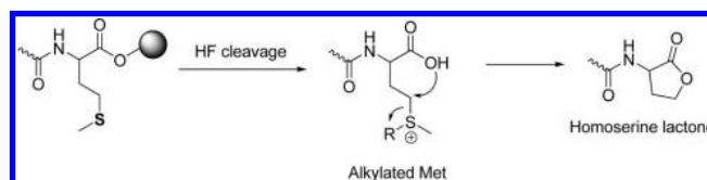
Figure 23. Homoserine lactone formation after Met alkylation during HF cleavage in the Boc/Bn solid-phase strategy.
