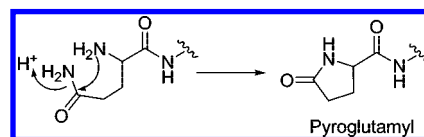
Figure 15. Pyroglutamyl formation.
