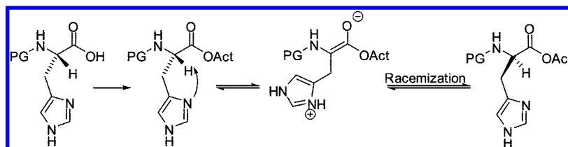
Figure 25. Proposed racemization mechanism of His during the coupling step .
